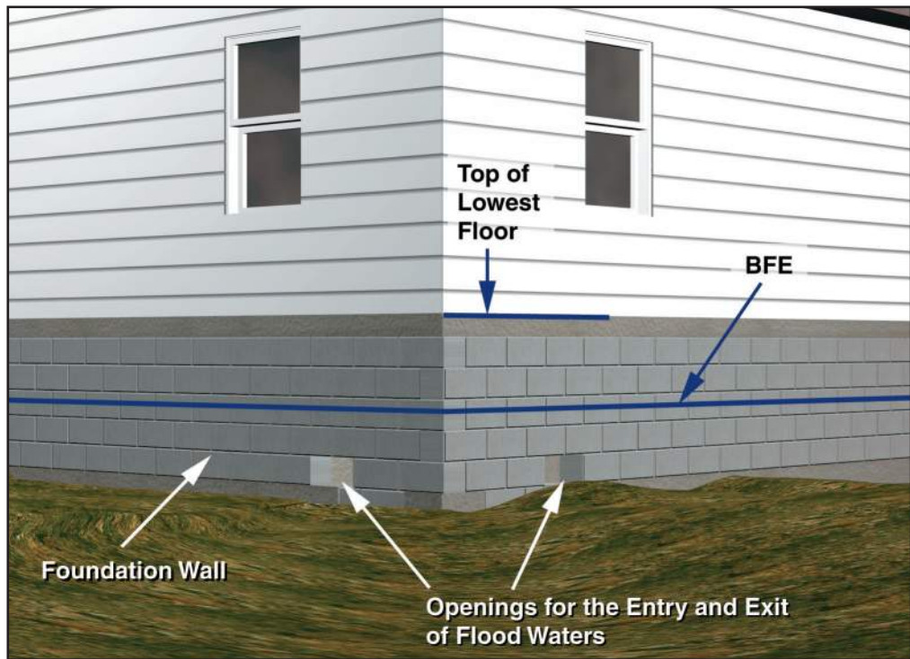
Figure 6 In a new, substantially improved, or substantially damaged building in an A zone, the elevation of the lowest floor must be at or above the BFE.
