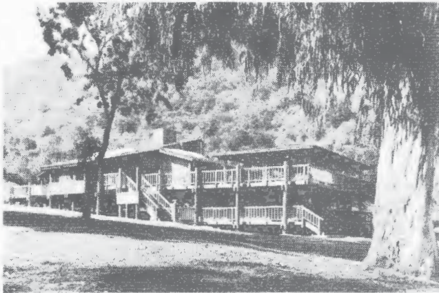
Figure 3.25. This wood structure successfully uses the same material throughout the building—foundation, structure, treatment of railings, wall, and roof material, as well as connection and anchorage details. The design honestly expresses the structure, foundations and other building elements. While it is obvious this is an elevated structure, it still feels very much a part of the site. The foundation members are also integrated well with the building itself (see also Figures 3.54 to 3.57).
