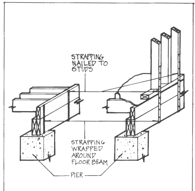
Figure 4.43. Metal Strapping
