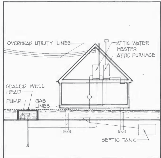
Figure 4.50. Locating Utilities
