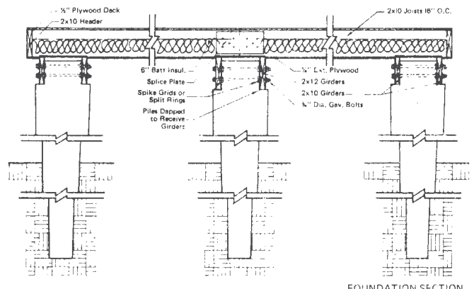
FOUNDATION SECTION
