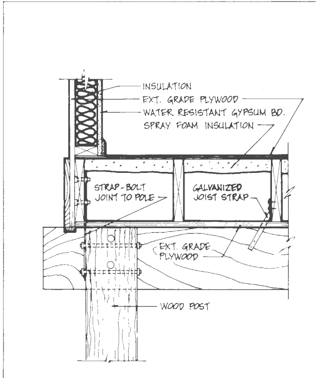
Figure 4.51. Insulated Floor Section, Wood Post Foundation
