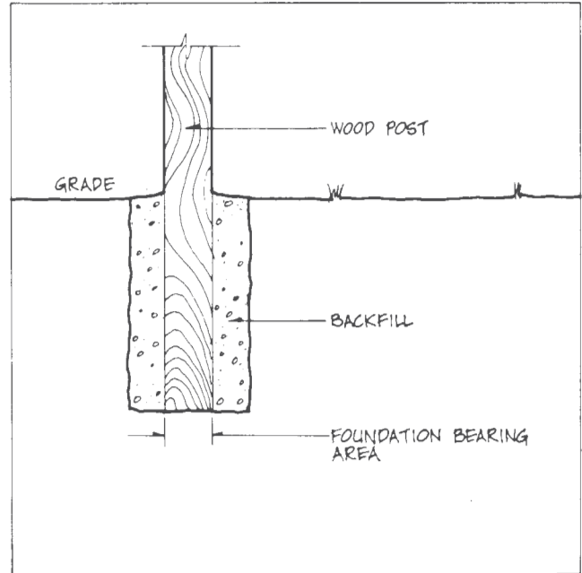
Figure 4.6. Earth Bearing
