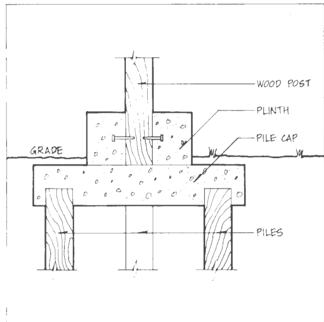
Figure 4.8. Post/Pile Foundation
