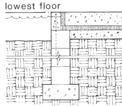
Figure 1.3. Elevation Requirements for Slab Foundations
