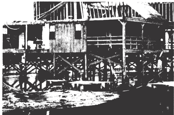
Figure 4.23. Diagonal Bracing
