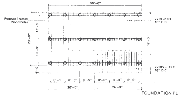
FOUNDATION PLAN
