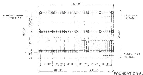
FOUNDATION PLAN
